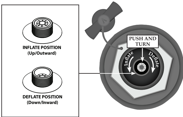
Figure 1. Inflate/ Deflate Spring Valve
