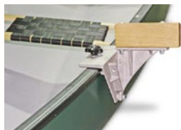
Sidekick Motor Mount
